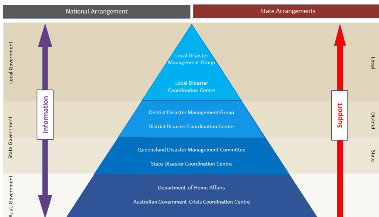
Figure 2: QDMA Triangle
