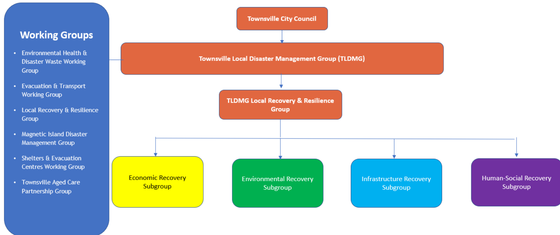
Figure 5: LDMG structure
