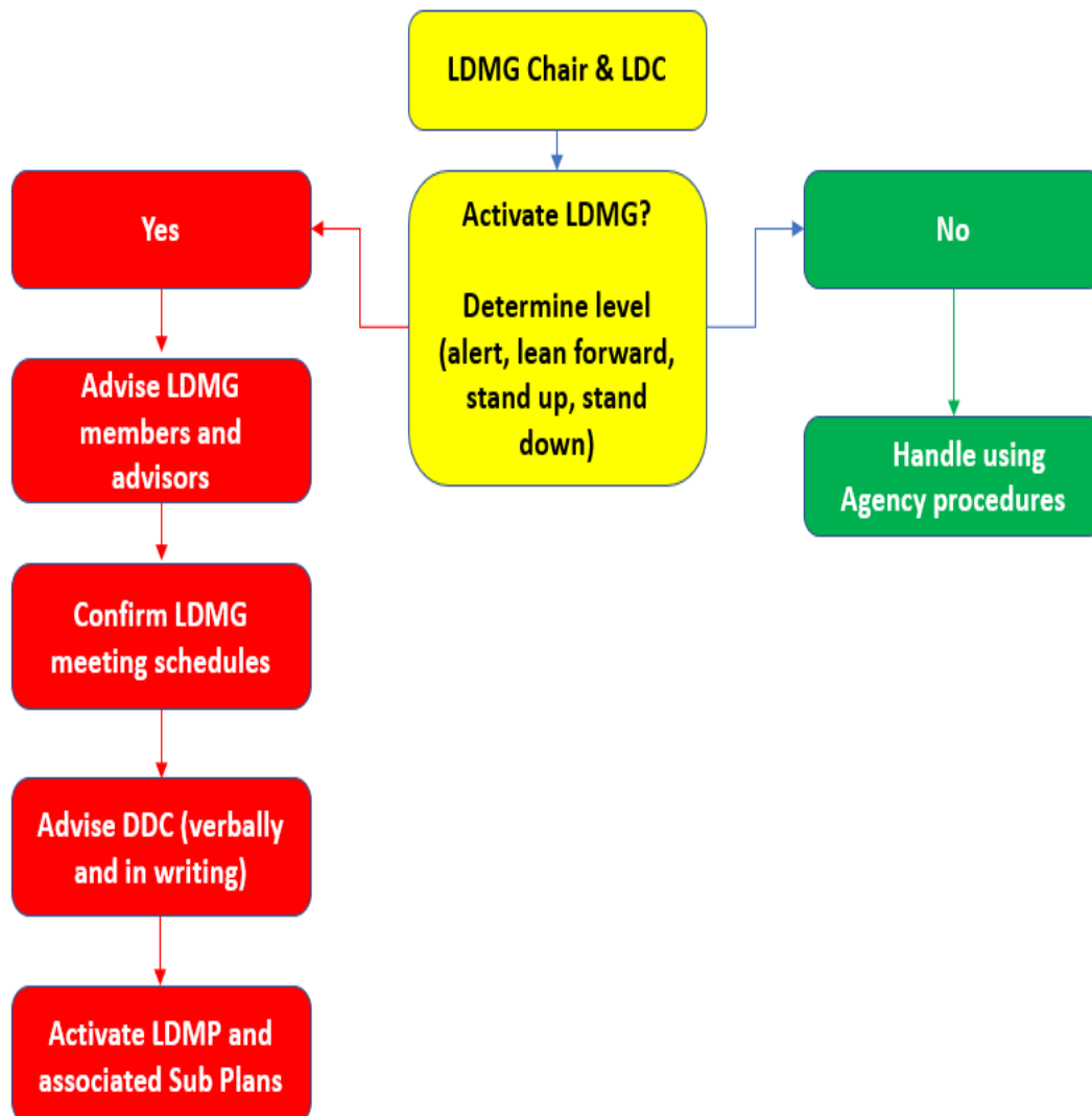
Figure 8: Notification flowchart
