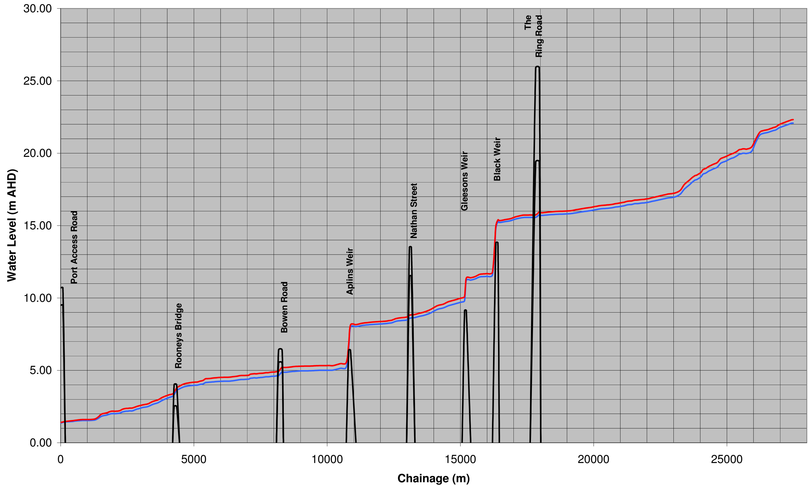
Figure C-2 Ross River Hydraulic Grade Line 50 and 100 Year ARI
