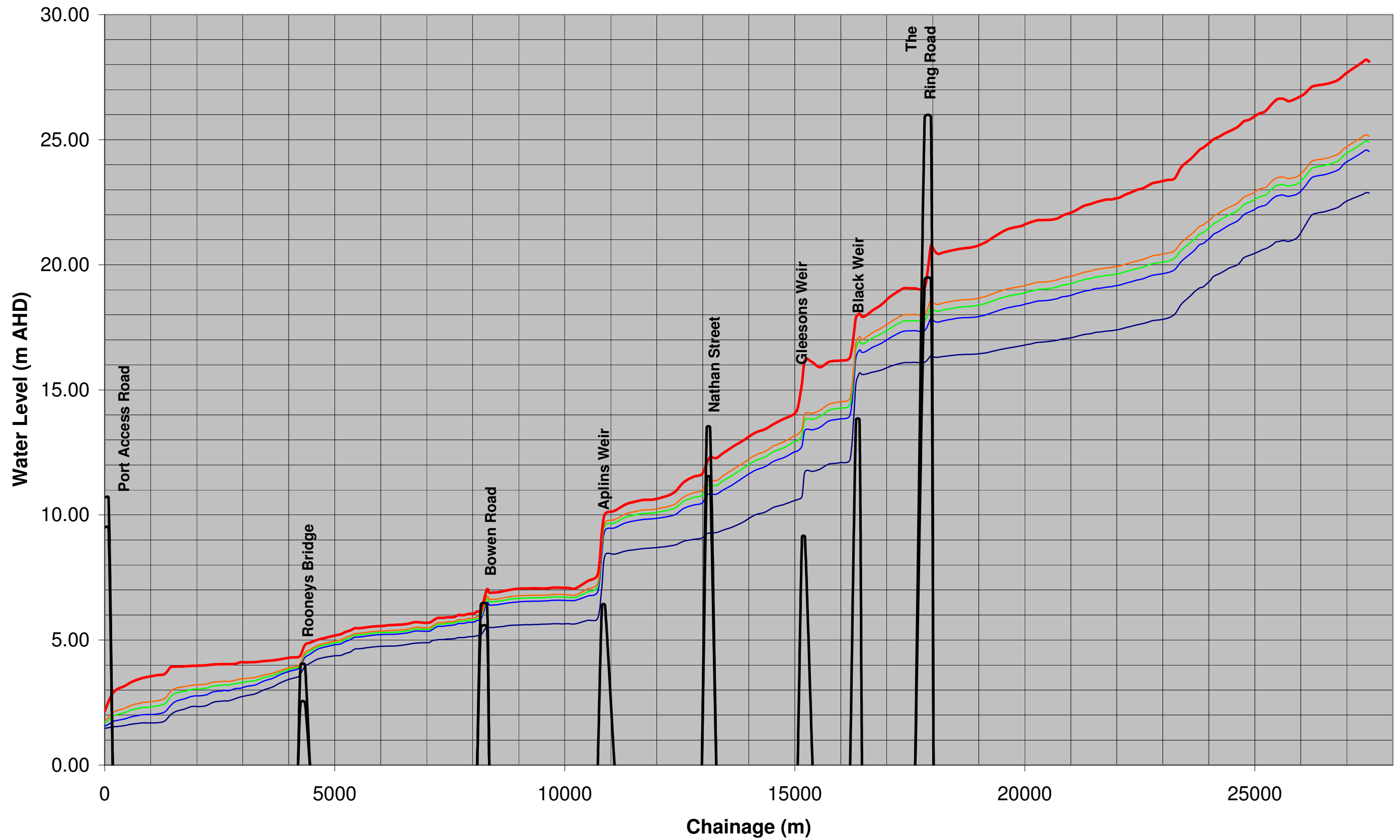
Figure C-3 Ross River Hydraulic Grade Line 200, 500, 1000, 2000 Year ARI and PMF, 72 hour event
