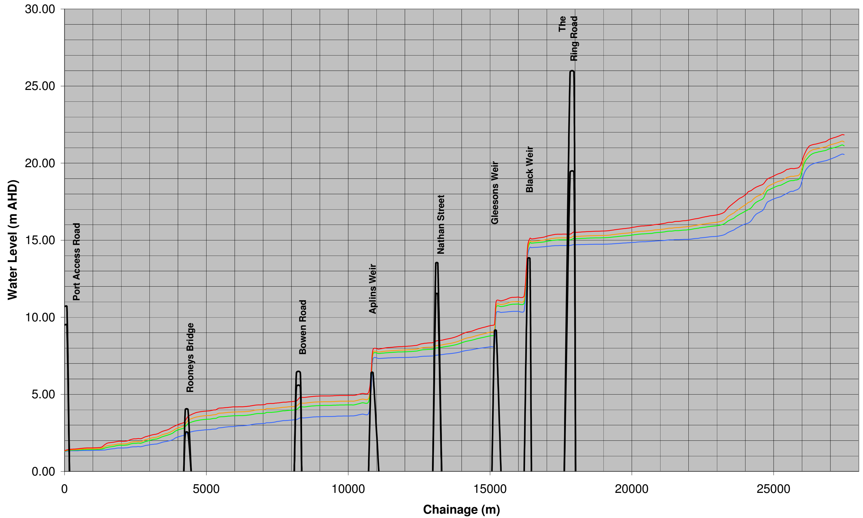
Figure C-1 Ross River Hydraulic Grade Line 2, 5, 10 and 20 Year ARI, 72 hour event
