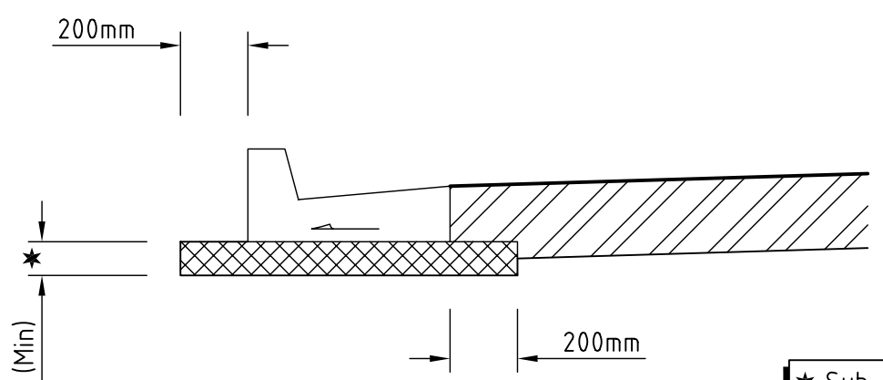
Detail 1 Pavement Depth \leq 250mm Type K \leq 265mm Type A/B NTS
