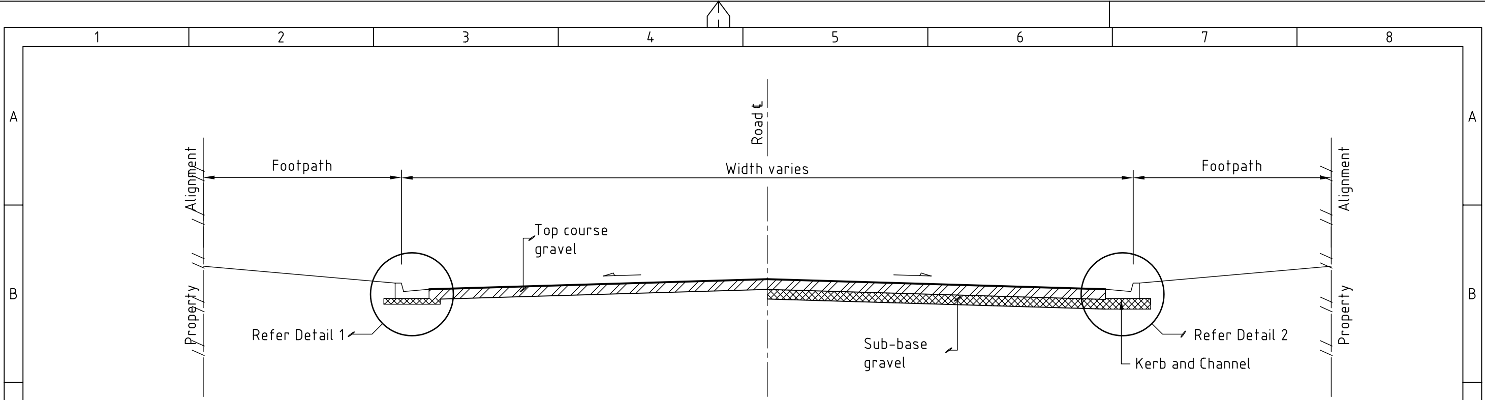
Type Cross Section NTS
