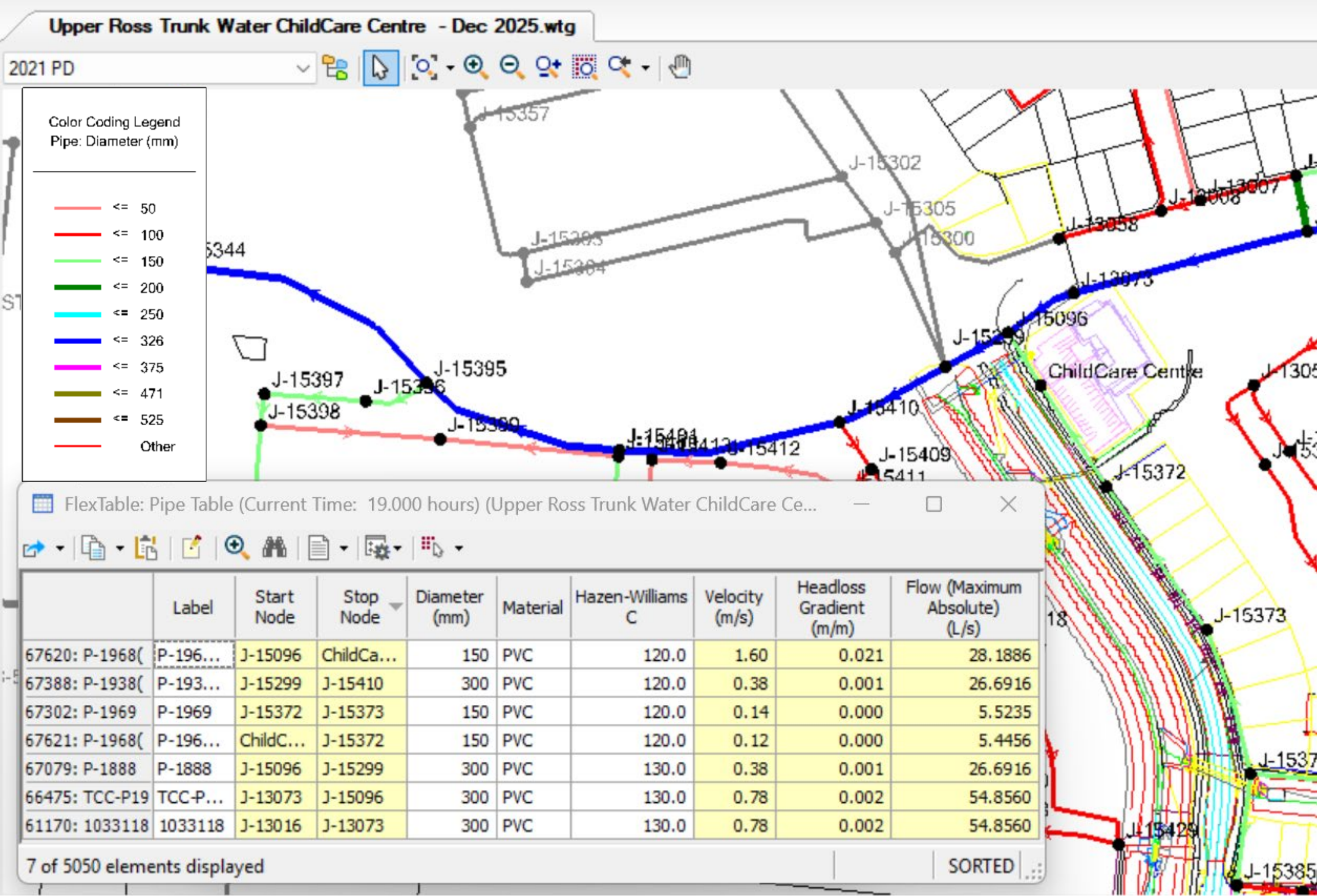
Rasmussen Early Learning Centre - Pipes Peak Hour & 30 l/s Fire Flow (7pm)
