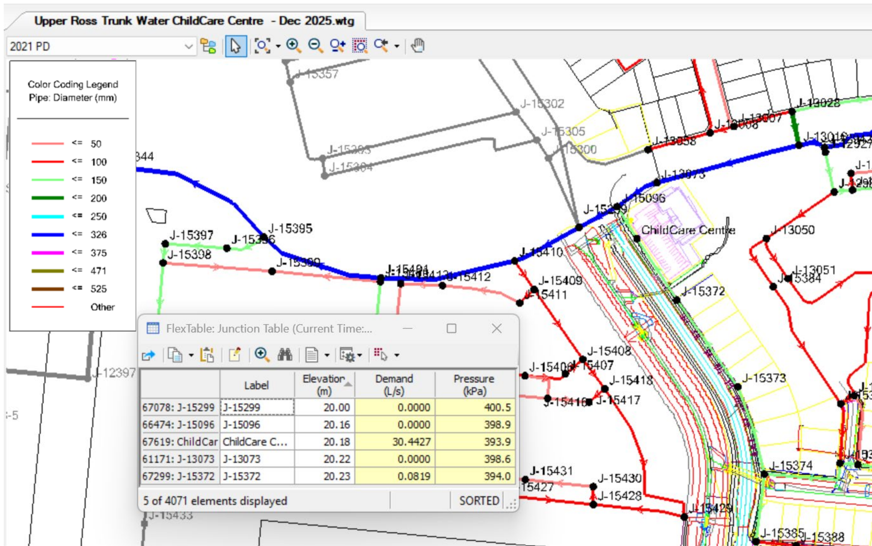
Rasmussen Early Learning Centre - Peak Hour Pressures & 30 l/s Fire Flow (12 noon)
