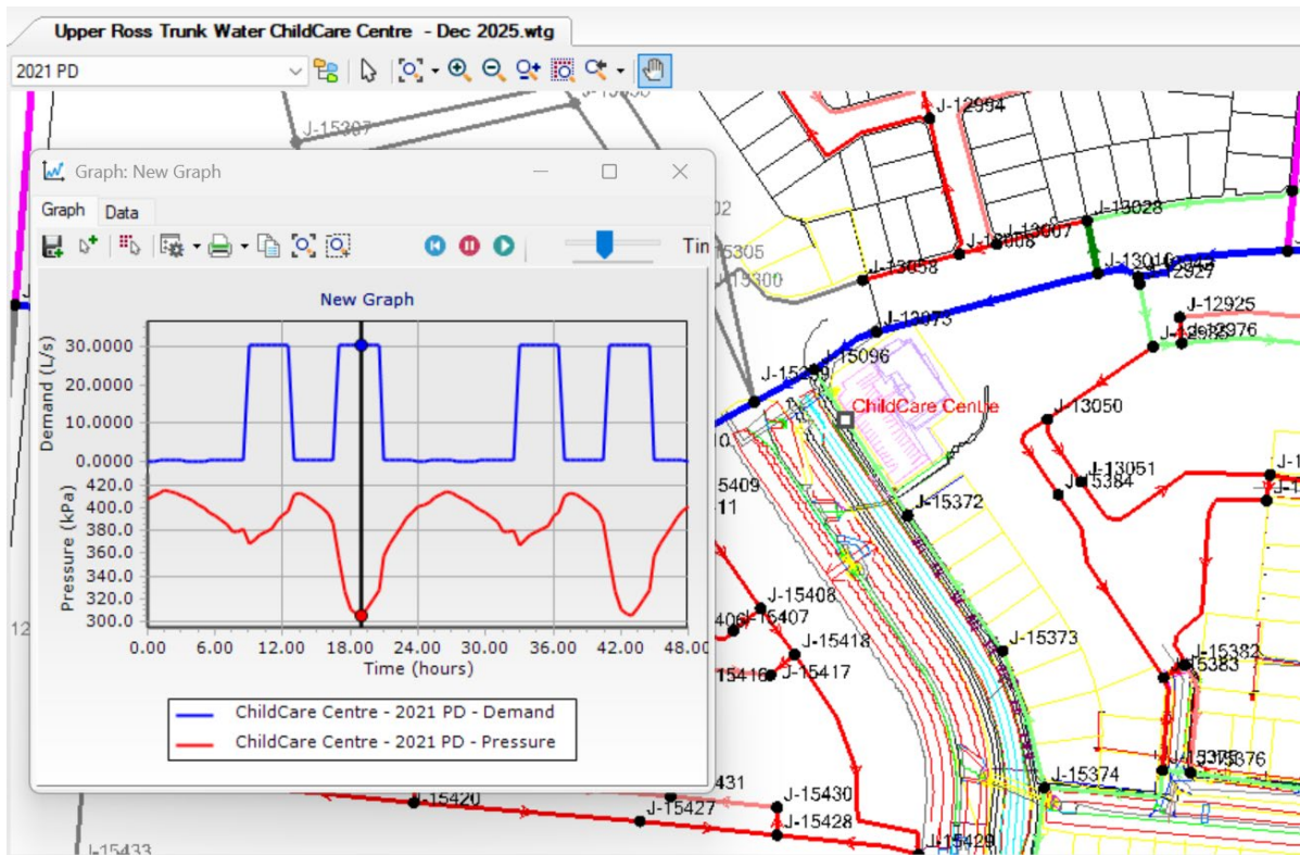
Figure 3.3 – Early Learning Centre Fire Flow Water Demands
