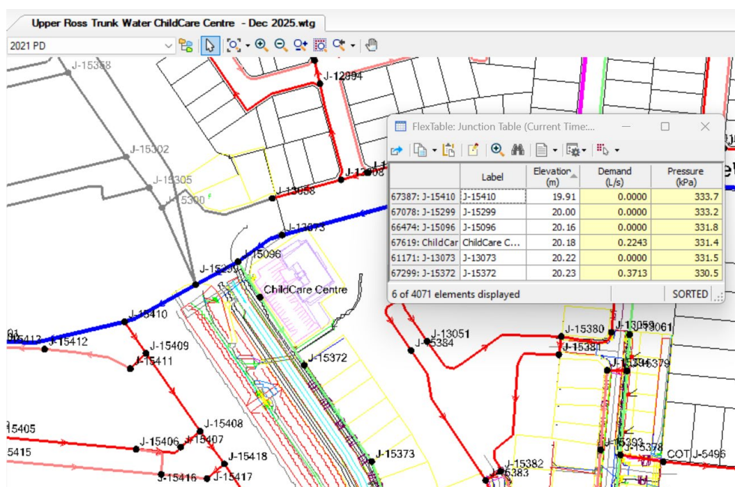
Figure 3.4 – Early Learning Centre Water Modelling & Pressures
