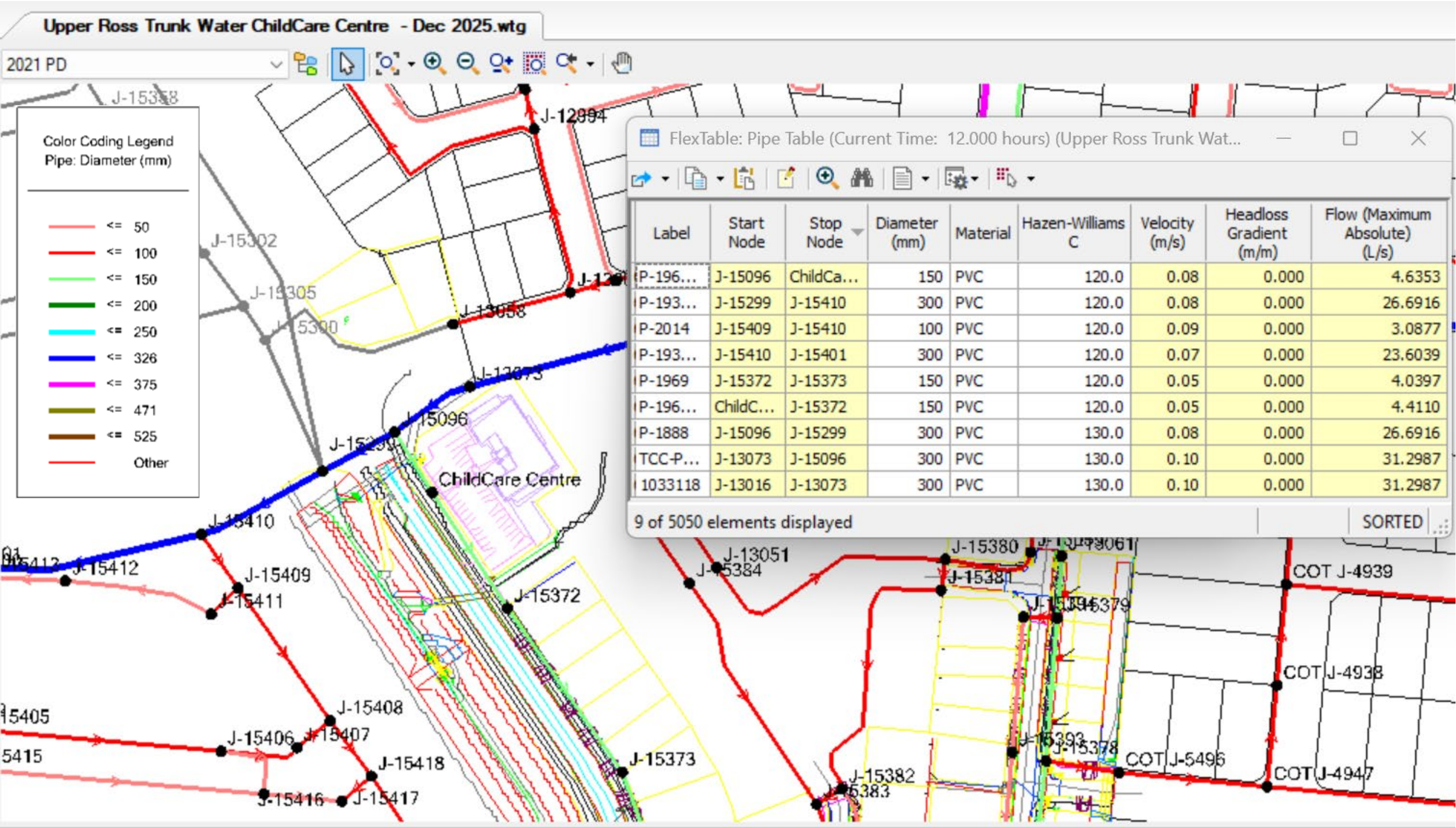
Rasmussen Early Learning Centre - Pipes Peak Hour Flows (12 noon)
