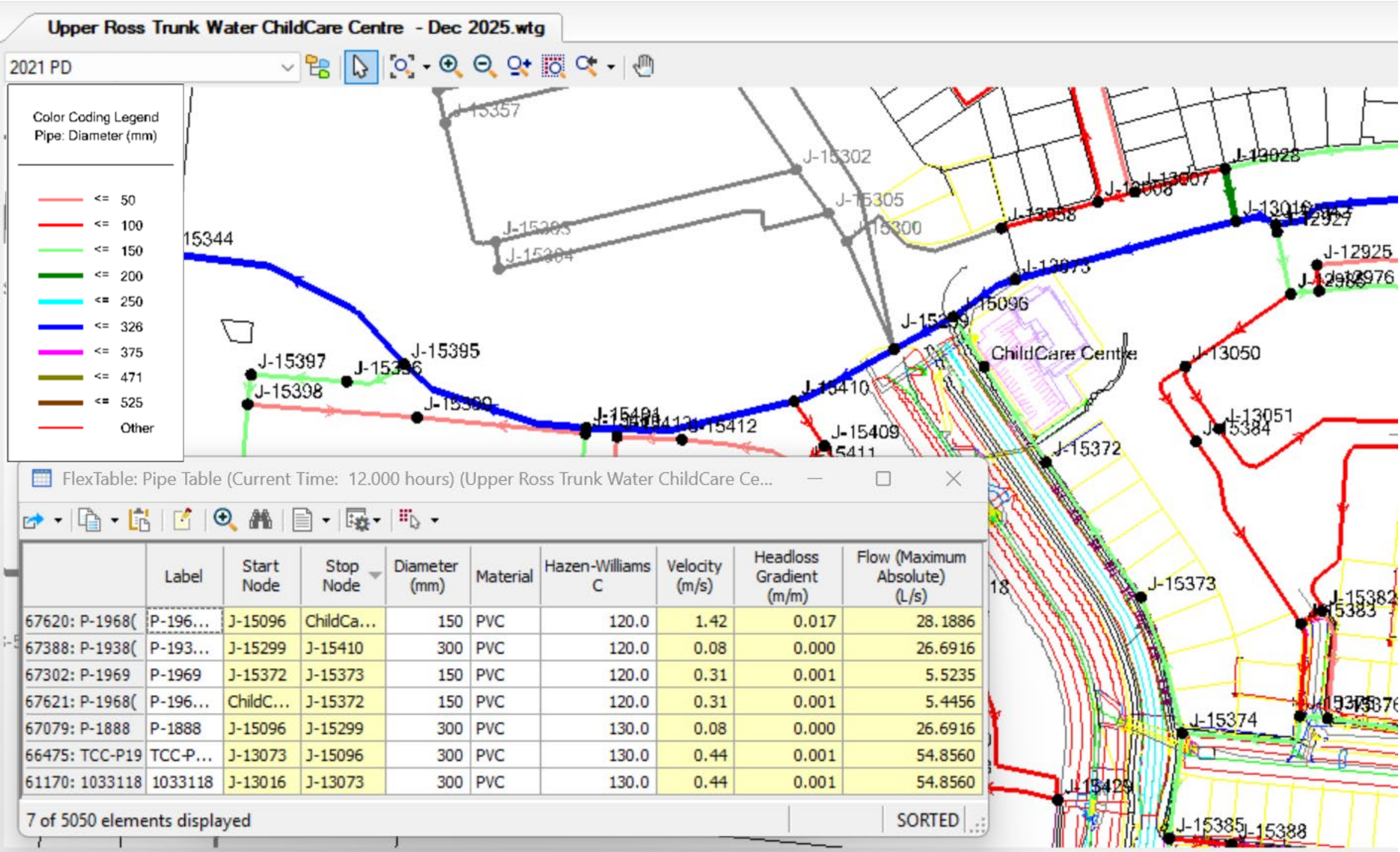
Rasmussen Early Learning Centre - Pipes Peak Hour & 30 l/s Fire Flow (12 noon)
