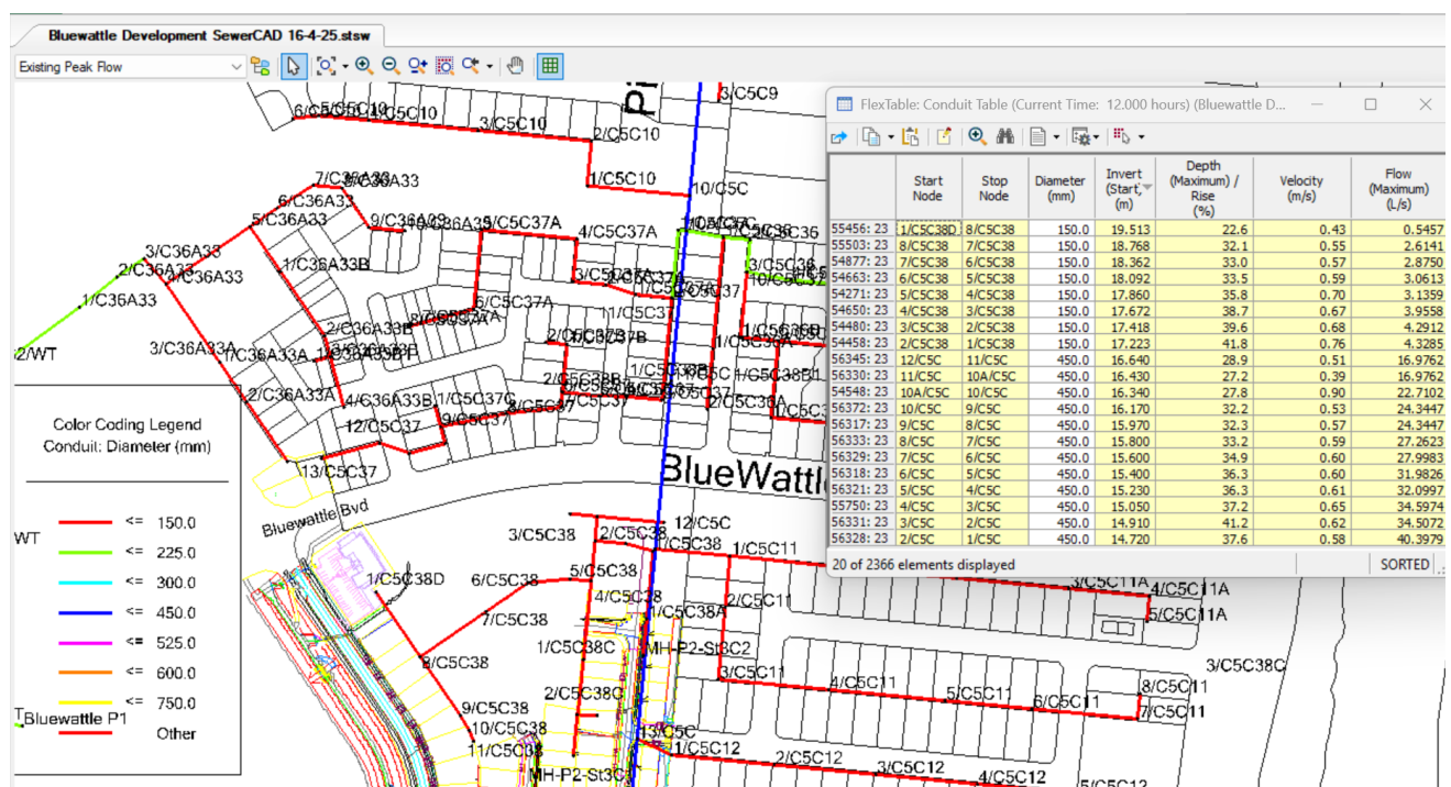
Figure 4.3 – SewerGEMS Modelling Results
