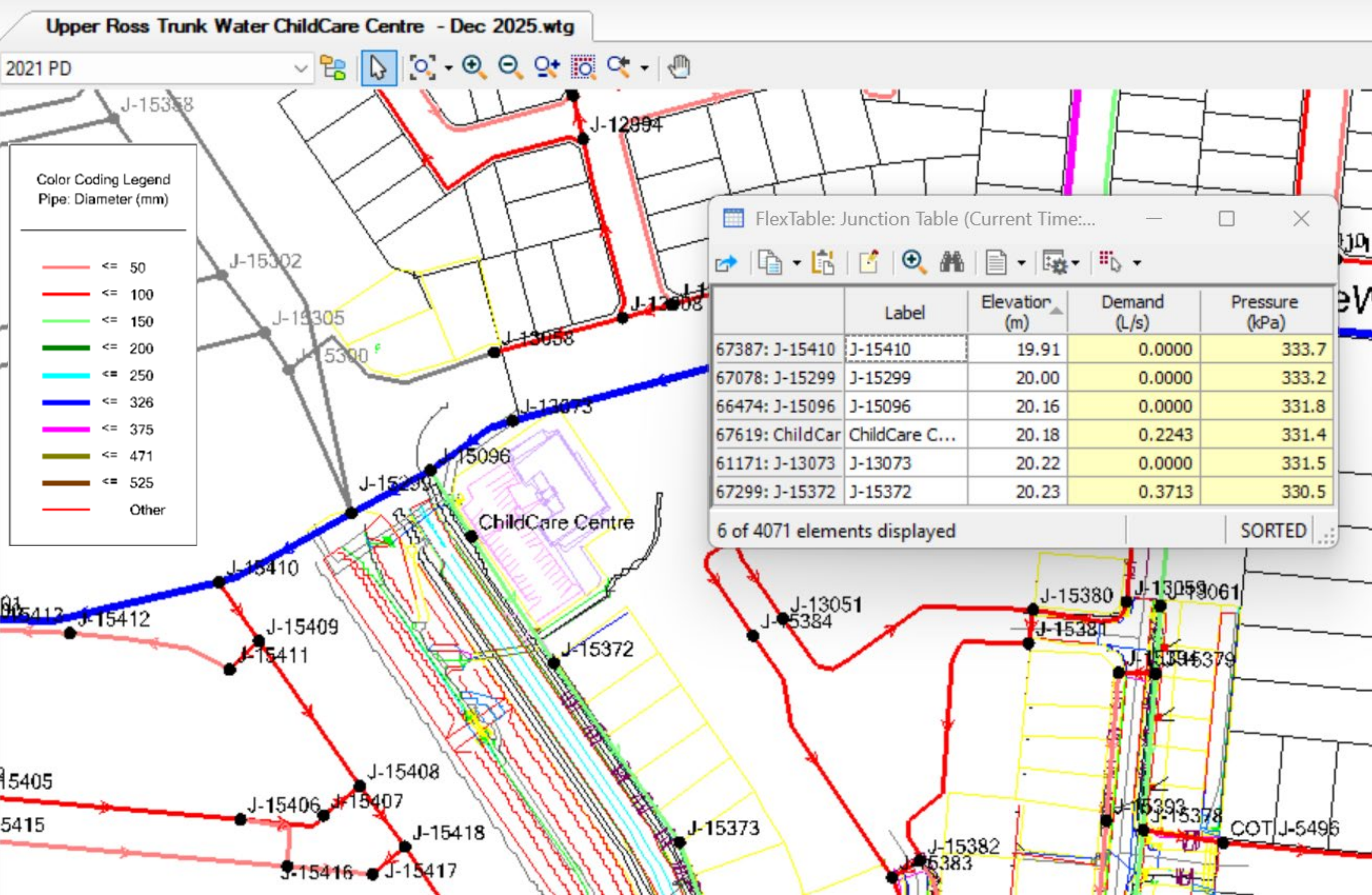
Rasmussen Early Learning Centre – Peak Hour Pressures (7pm)
