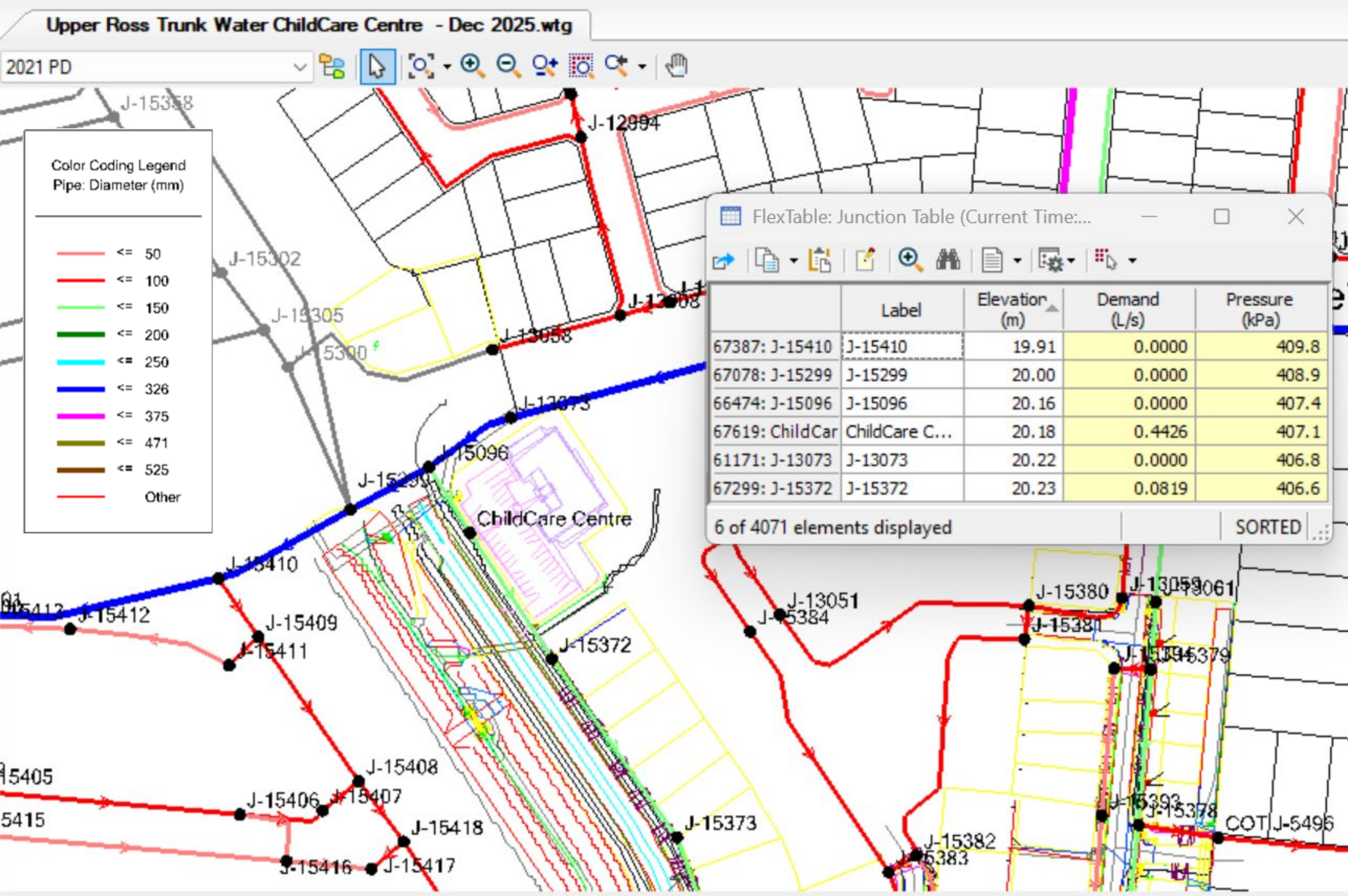
Rasmussen Early Learning Centre – Peak Hour Pressures (12 noon)
