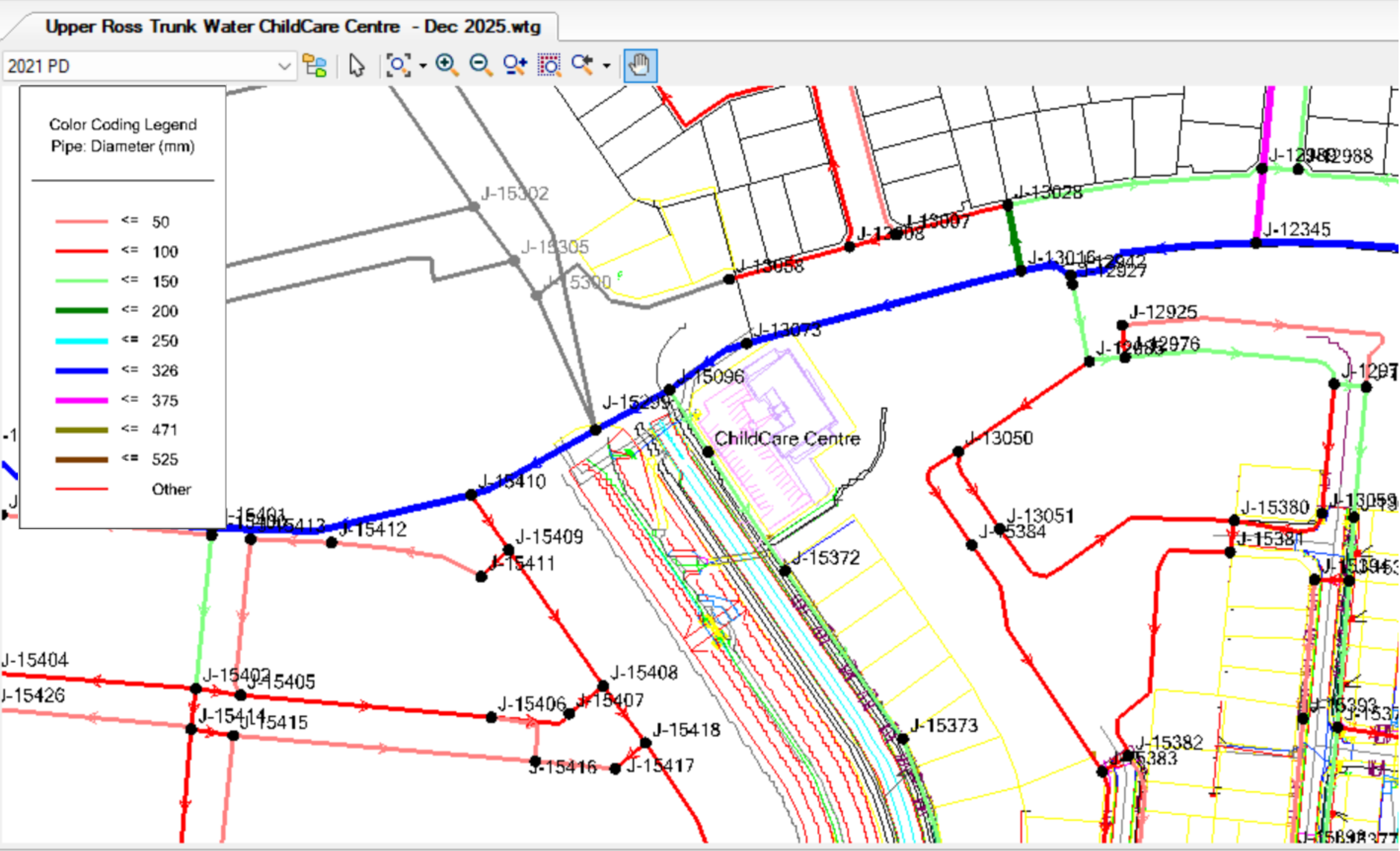
Rasmussen Early Learning Centre - WaterGEMS Model Figure
