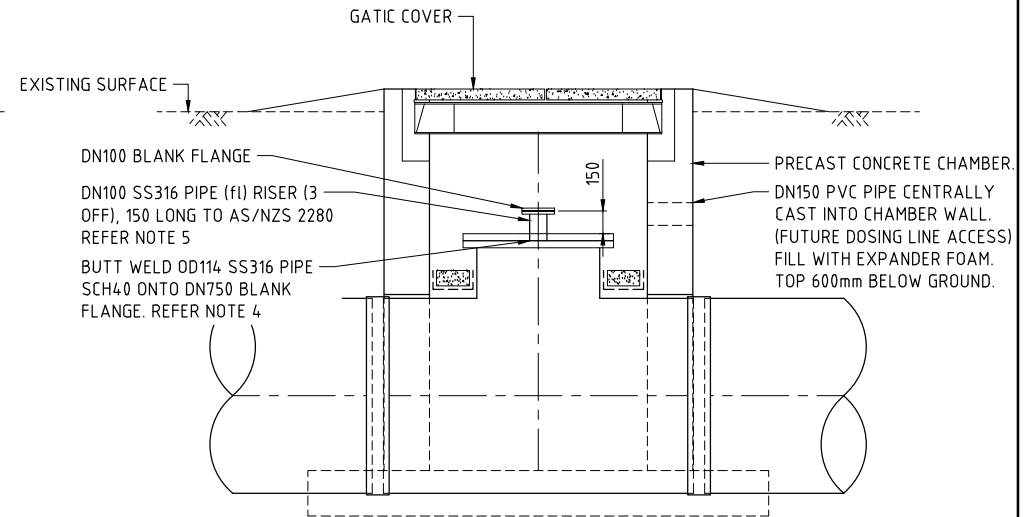
SECTION 2 DOSING MANHOLE INSTALLATION ARRANGEMENT SCALE G
