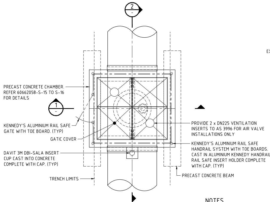
PLAN AIR VALVE INSTALLATION ARRANGEMENT SCALE G
