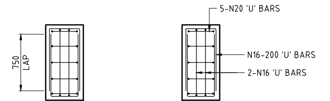
SECTION 5 SCALE G
