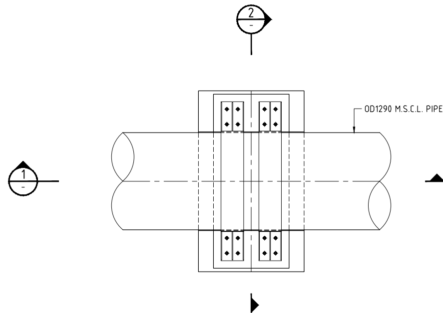
PLAN PIPE PEDESTAL ARRANGEMENT SCALE G
