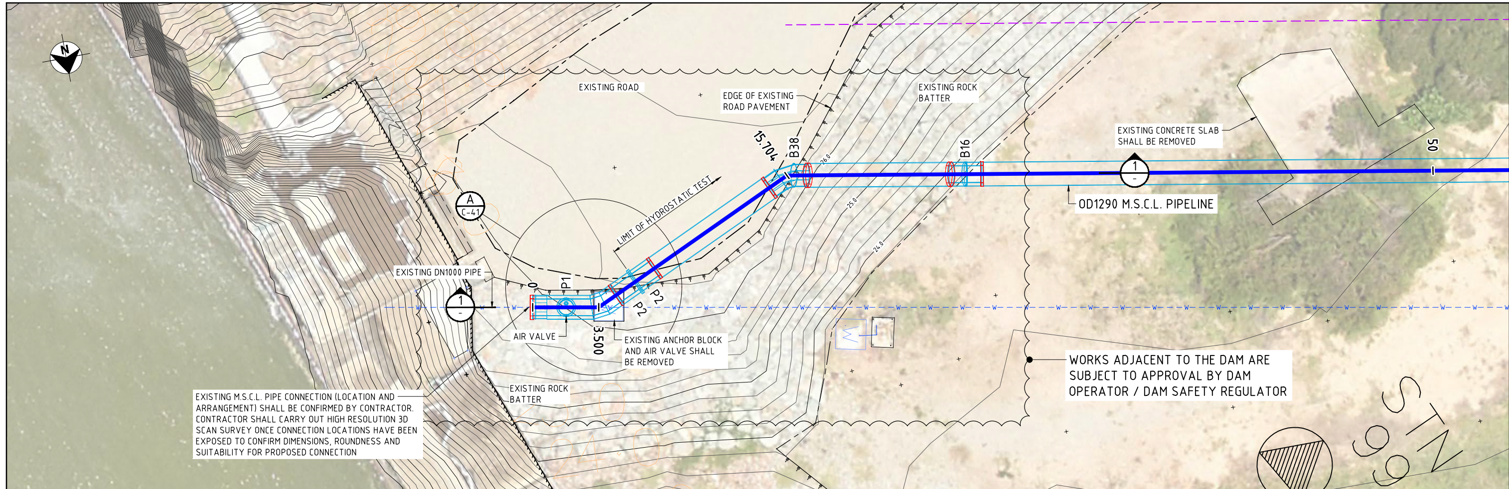
PLAN
