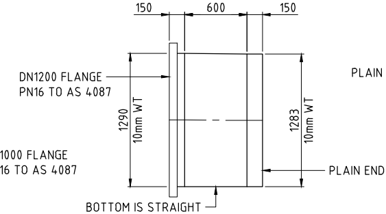
MK RE5 - ELEVATION
