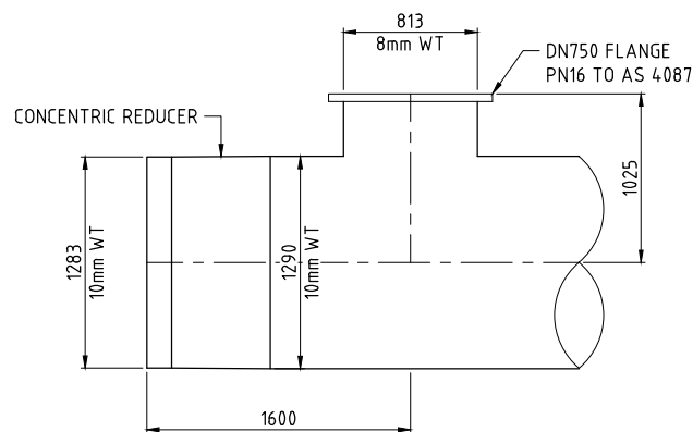
SECTION 1
