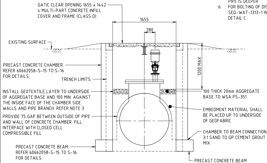
SECTION 1 SCALE G
