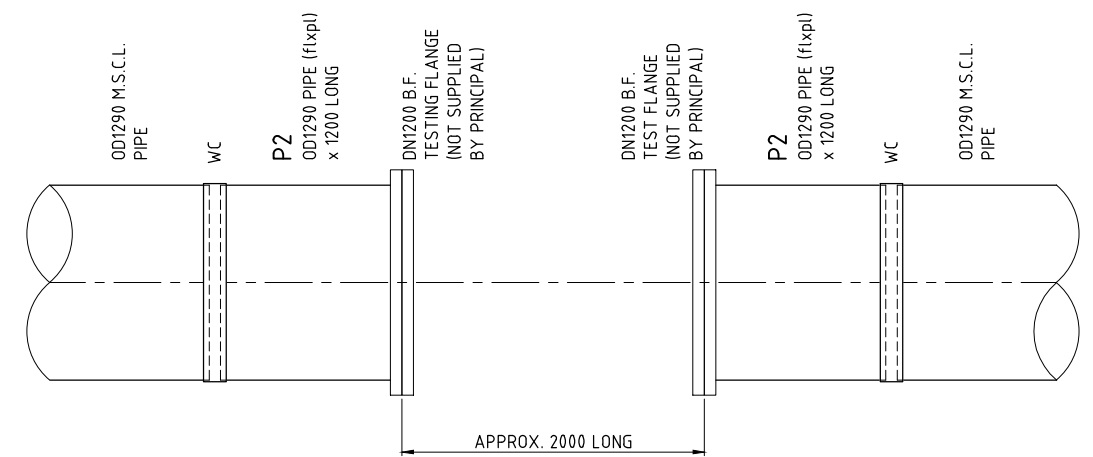
PLAN HYDROSTATIC TEST LOCATION TESTING PIPEWORK CONFIGURATION SCALE G
