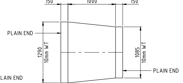
MK RC1 - ELEVATION
