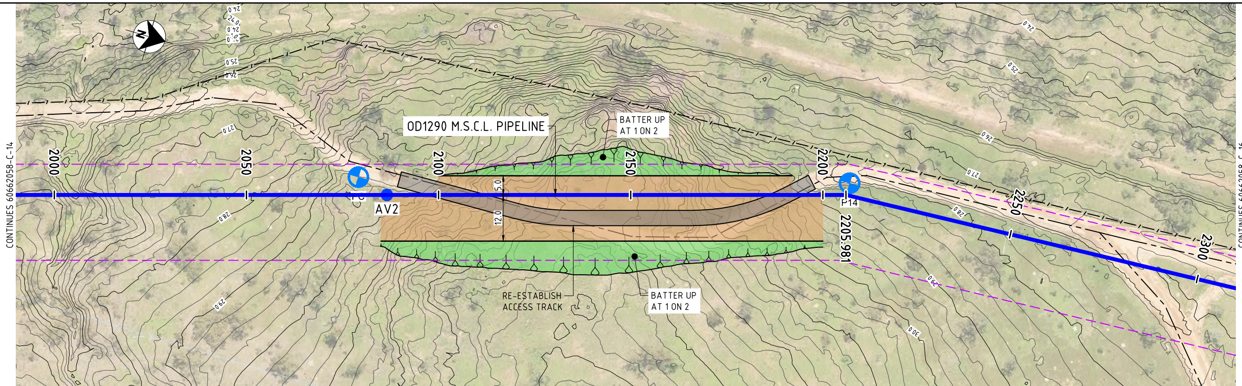
PLAN
