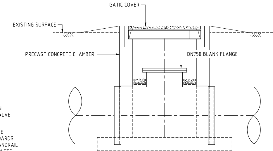
SECTION 2 ACCESS MANHOLE INSTALLATION ARRANGEMENT SCALE G
