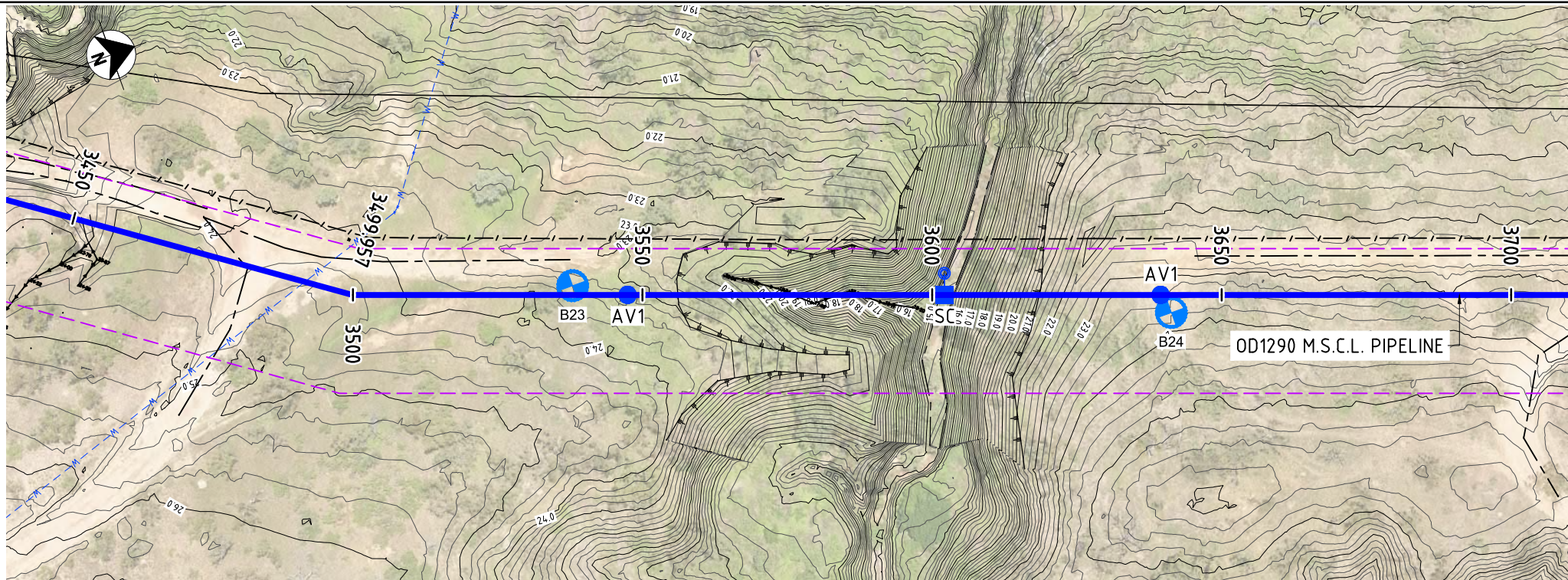
PLAN
