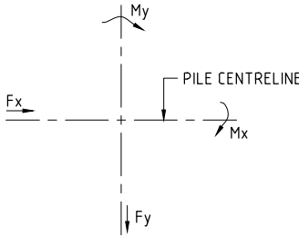
SHEAR FORCE AND BENDING MOMENT DIAGRAM
