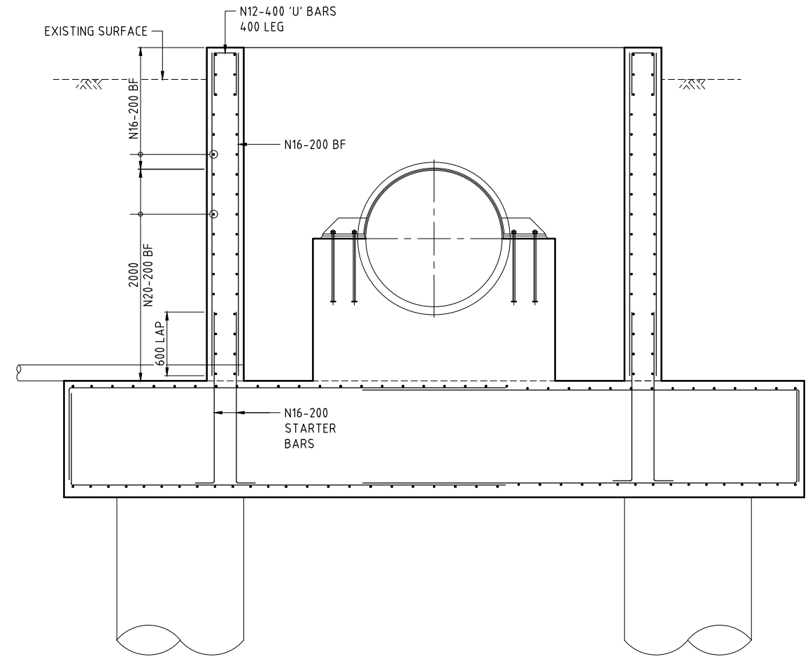
SECTION 5 SCALE G
