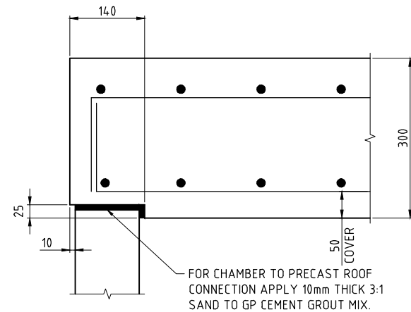
SECTION 1 SCALE K CHAMBER TO PRECAST ROOF CONNECTION
