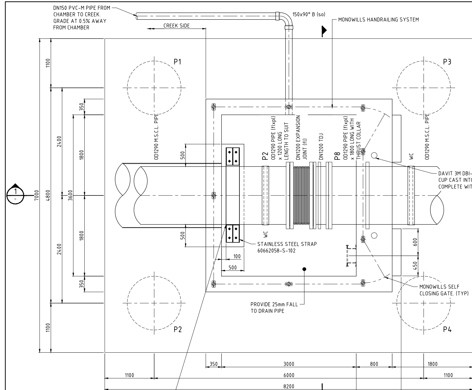
6mm THICK x 1500mm WIDE RUBBER WRAPPED AROUND PIPE CENTRALLY LOCATED ON EACH PEDESTAL. FIX TO PIPE IN ACCORDANCE WITH MANUFACTURERS RECOMMENDATIONS. 6mm THICK x 1100mm WIDE PTFE SHEET SHALL BE WRAPPED AROUND PIPE CENTRALLY LOCATED ON EACH PEDESTAL BETWEEN RUBBER AND CONCRETE / STAINLESS STEEL STRAPS. PLAN EXPANSION JOINT INSTALLATION ARRANGEMENT SCALE G
