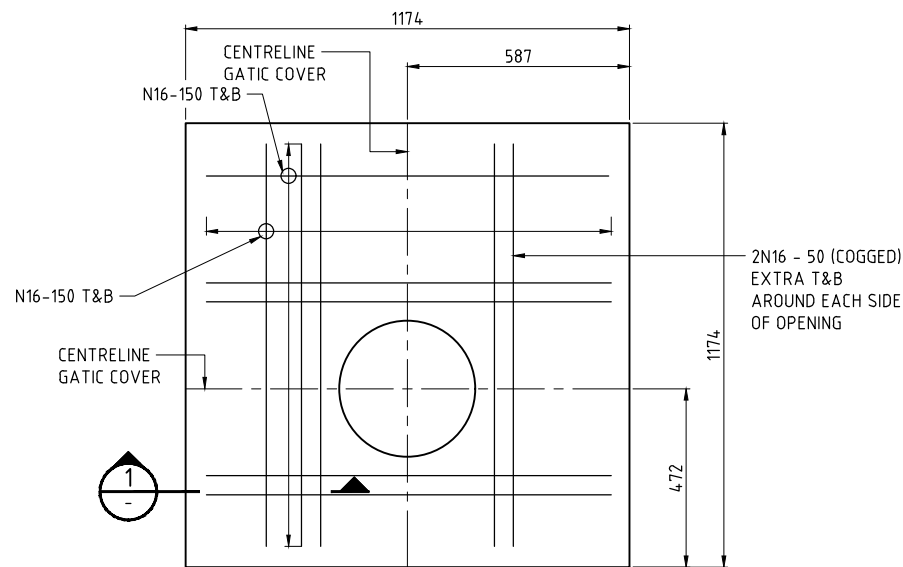
DETAIL B SCALE J PRECAST LID REINFORCEMENT DETAILS
