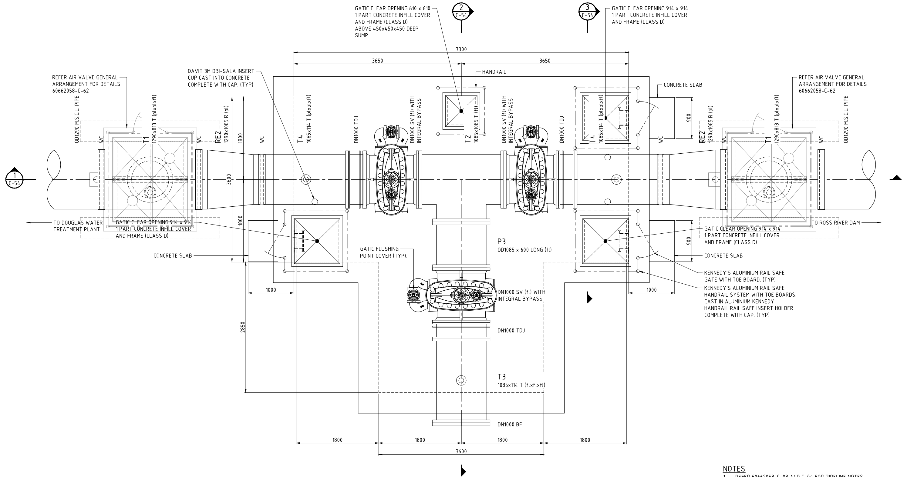
PLAN CH5731 - VALVE CHAMBER INSTALLATION ARRANGEMENT SCALE G 60662058-C-27
