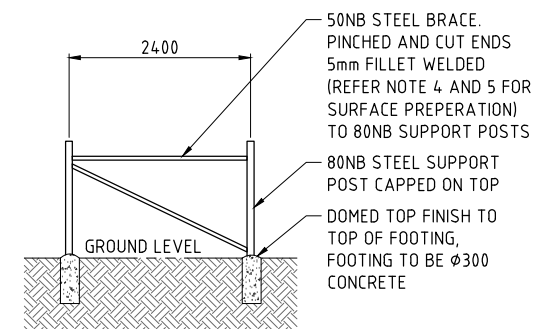
TYPICAL STRAINER POST ARRANGMENT
