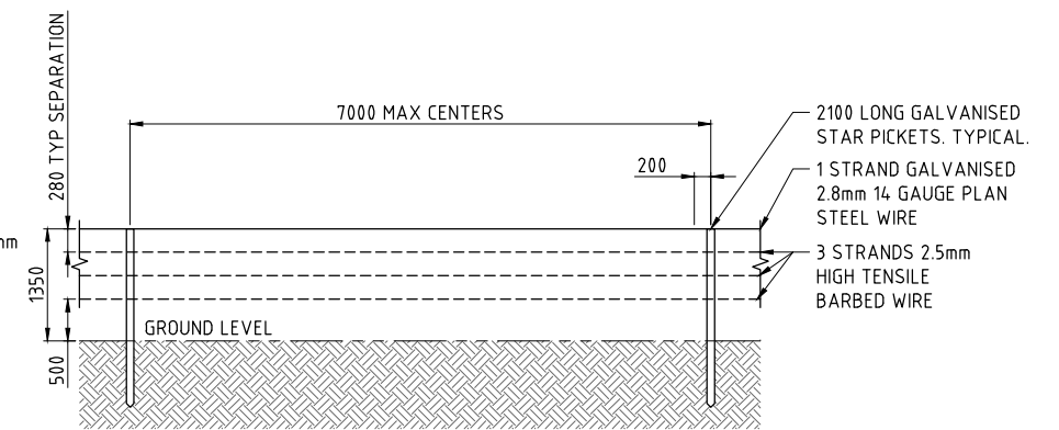
TYPICAL FENCE ARRANGMENT - 3 STRAND
