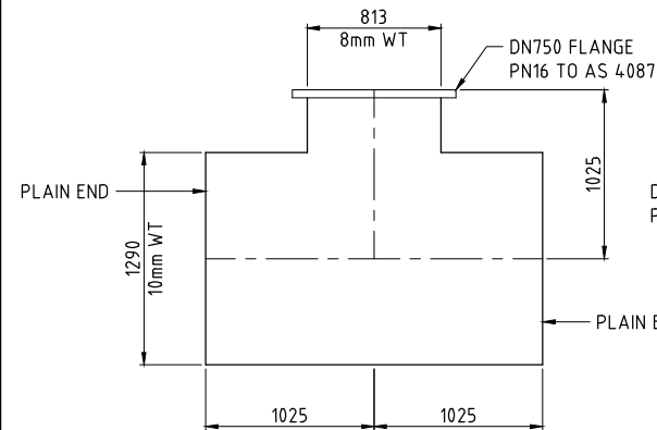
MK T1 - ELEVATION
