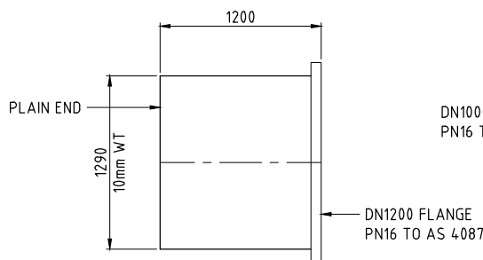
MK P2 - PLAN
