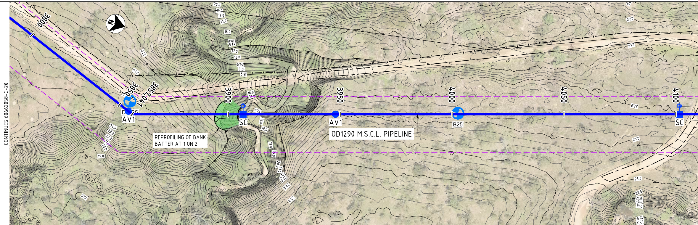
PLAN
