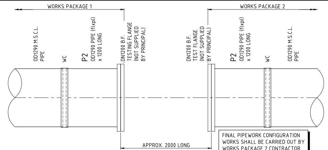
PLAN WORKS PACKAGES INTERFACE TESTING PIPEWORK CONFIGURATION SCALE G
