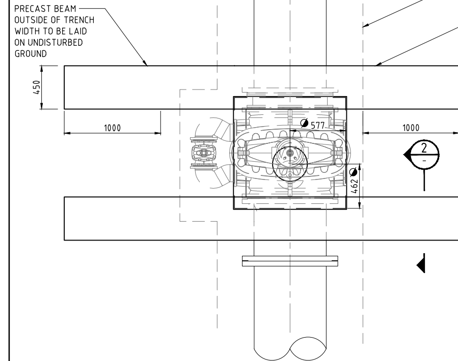
GATE VALVE INSTALLATION ARRANGEMENT (WITH INTEGRAL BYPASS) SCALE H
