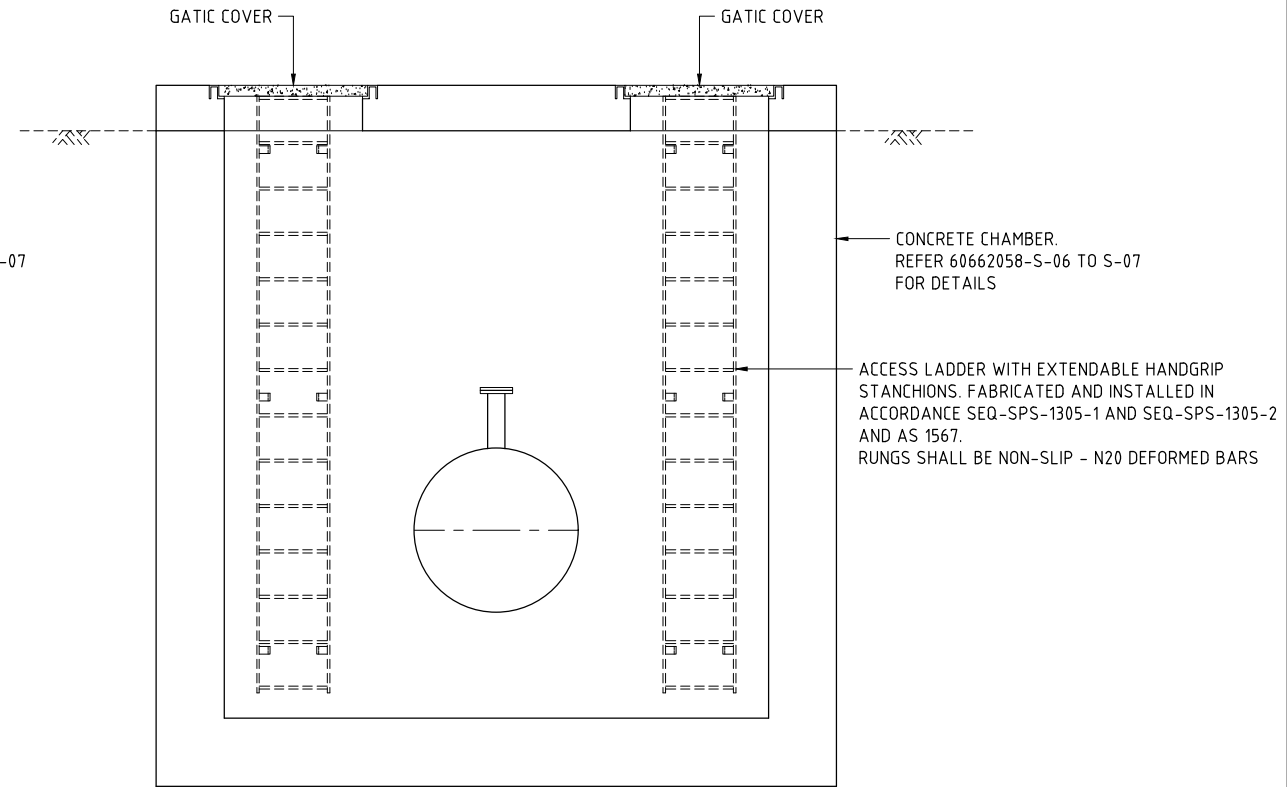
SECTION 3 SCALE G C-53
