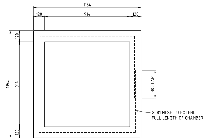
MAINTENANCE ACCESSIBLE PRECAST 914 x 914 CHAMBER SCALE J
