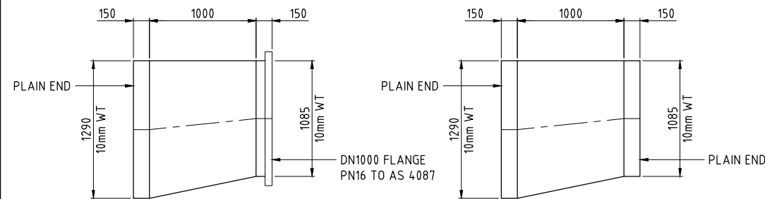
MK RE1 - ELEVATION
