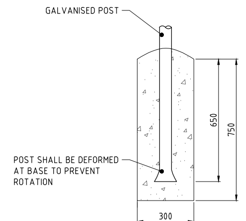
FOOTING DETAIL
