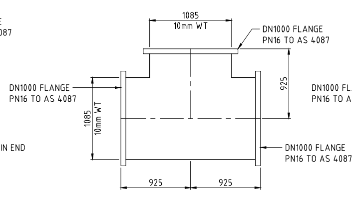
MK T2 - PLAN
