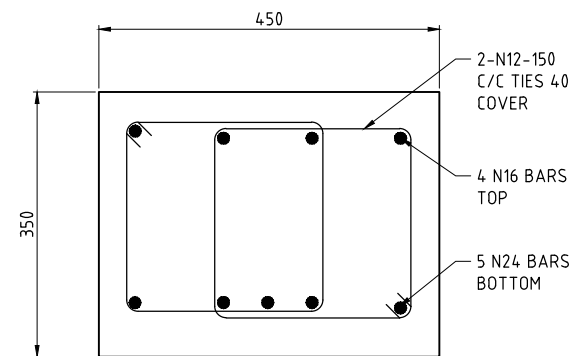
SECTION 2 SCALE J PRECAST BEAM REINFORCEMENT DETAILS
