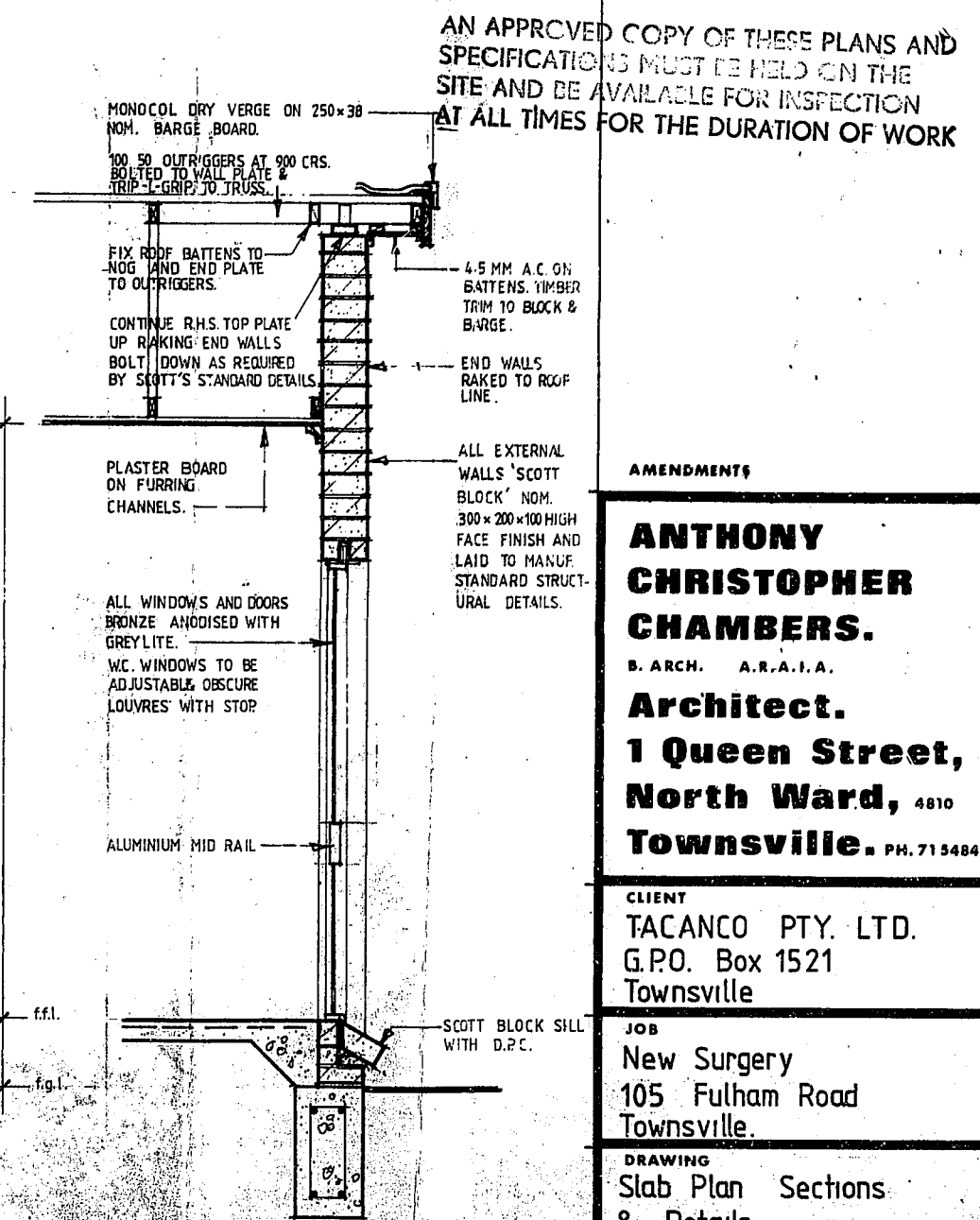
END WALL SECTION
