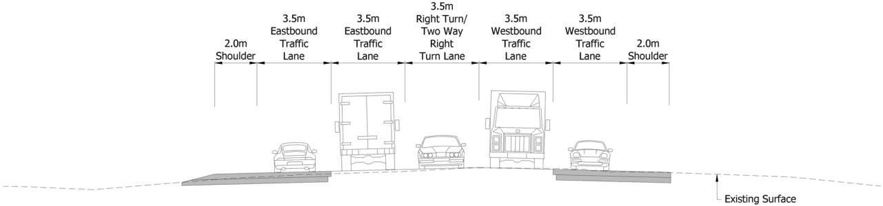
TYPICAL SECTION E TAFE TO CATALYST COURT
