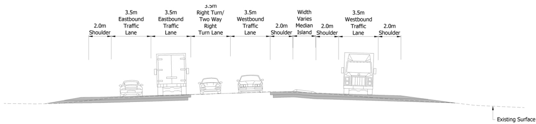
TYPICAL SECTION G GAZETTED INGHAM (NEW SLIP ROAD) TIE TO EXISTING INGHAM ROAD
