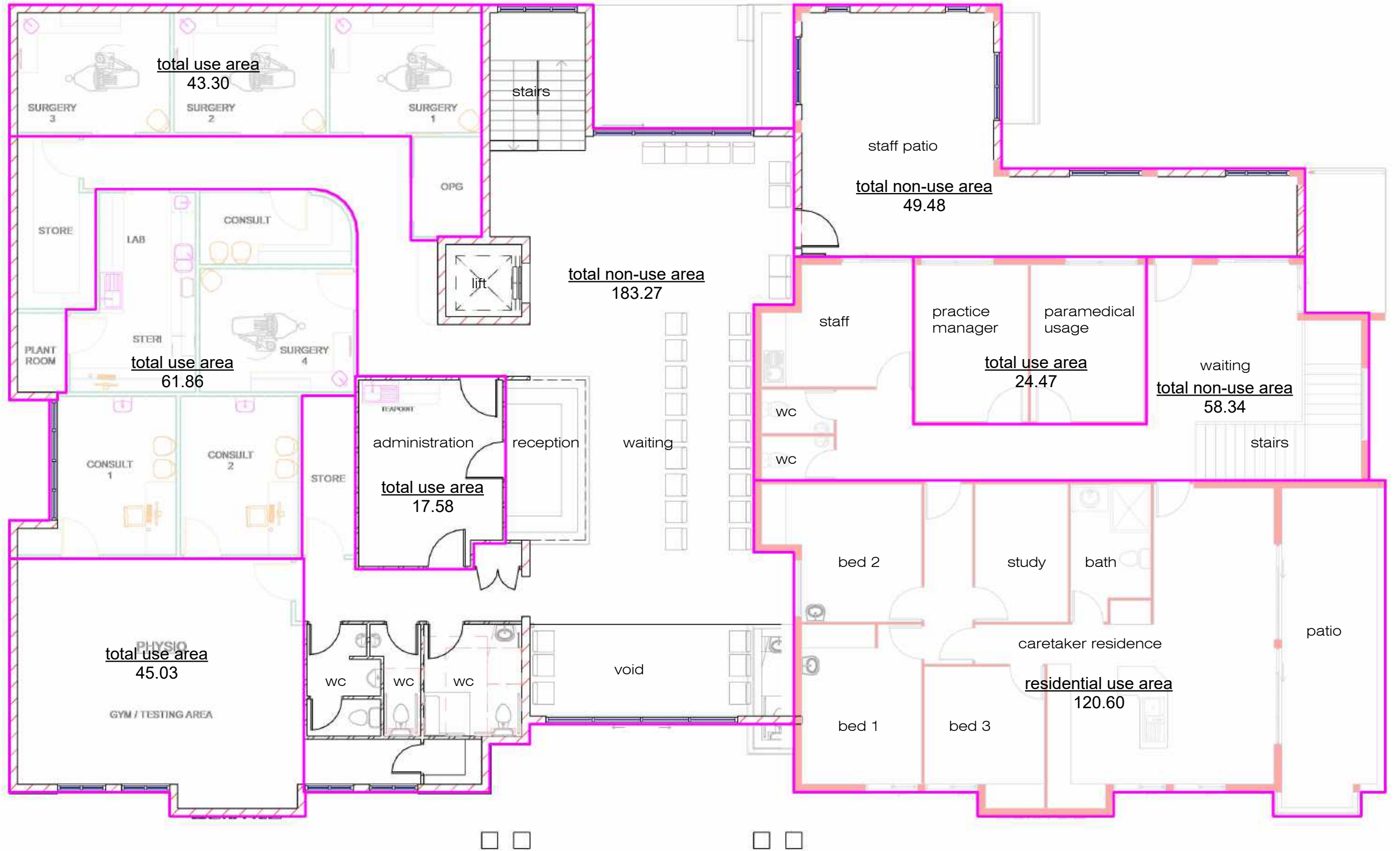
2 first floor level 1 : 100
