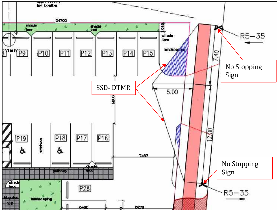
Figure 32. Required SSD based on DTMR and Approximate location of No Stopping Sign.
