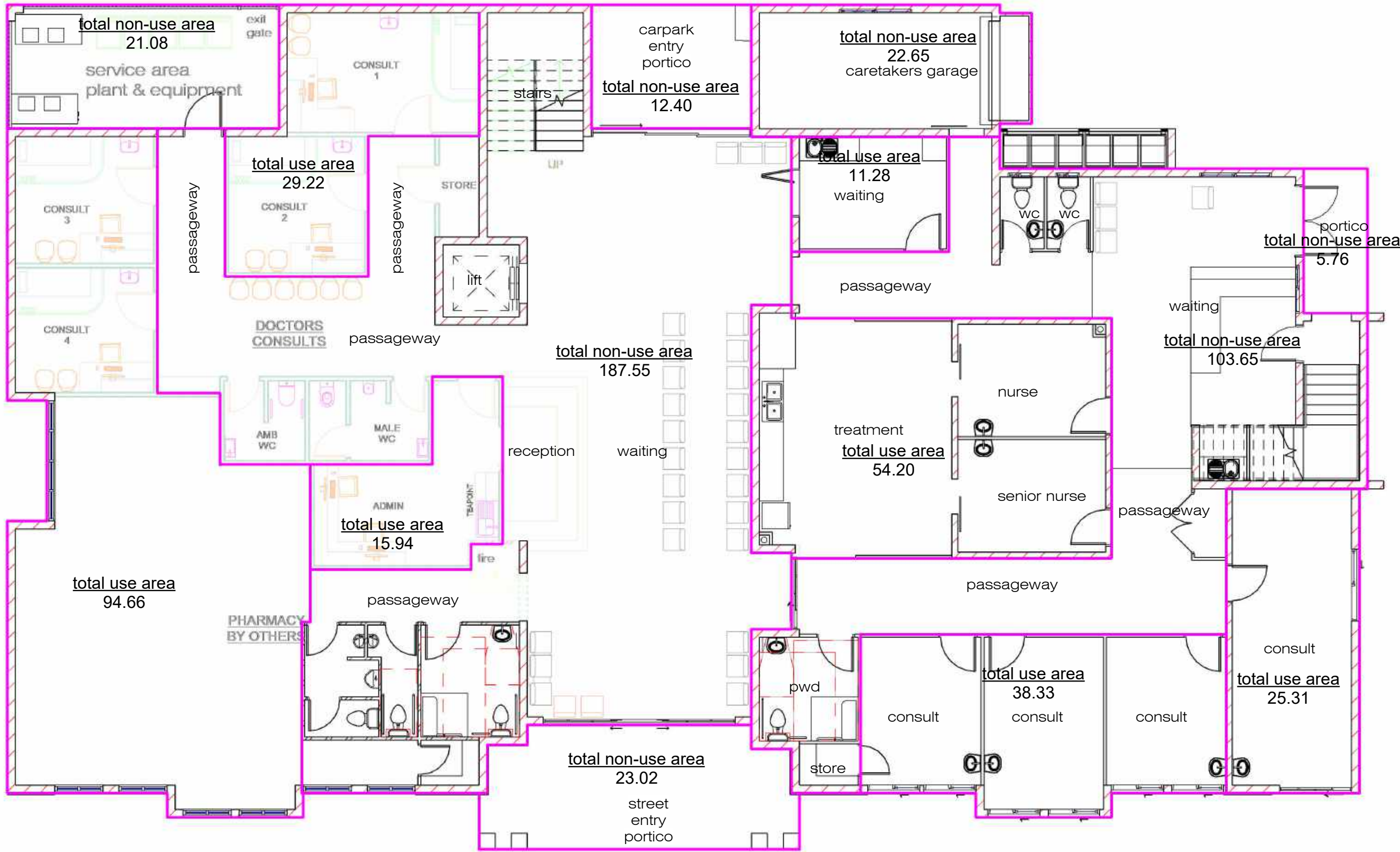
1 ground floor level 1 : 100
