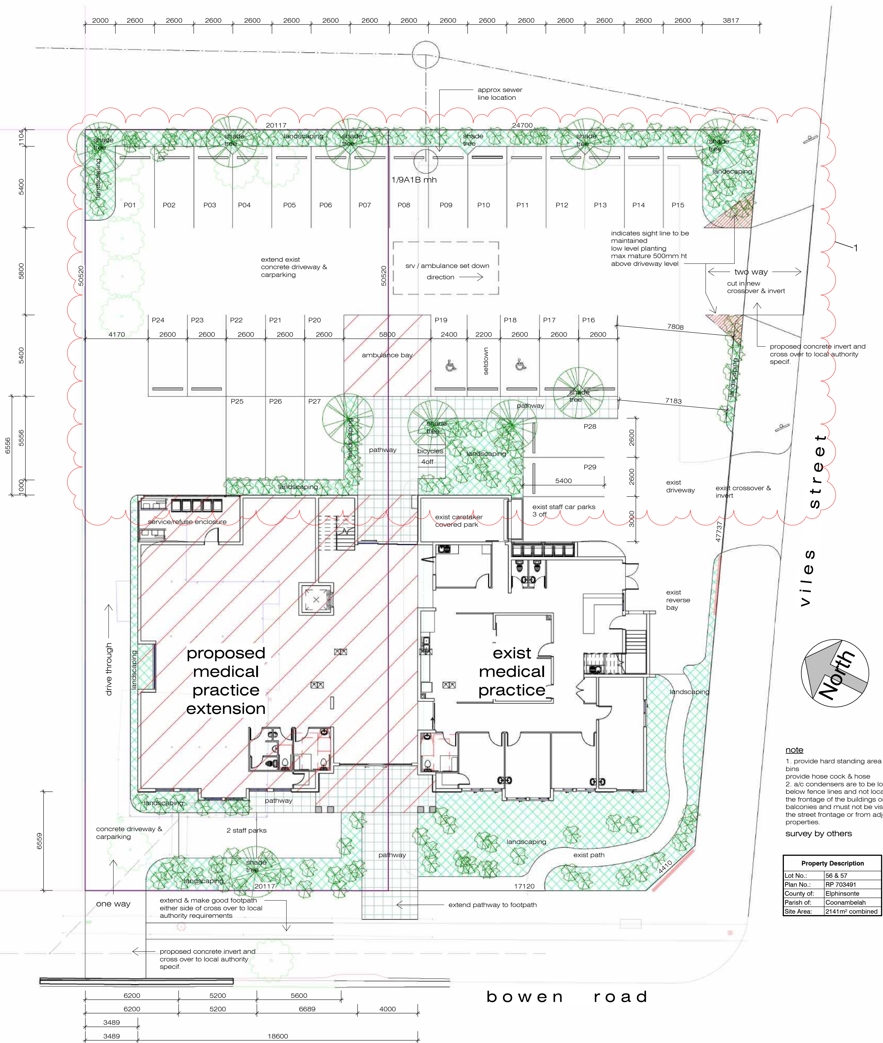
1 proposed site plan sk_02 1 : 150
